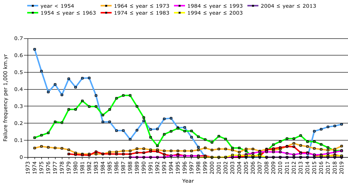
Figure 50: Failure frequency (five year moving average) of corrosion incidents and year of construction
