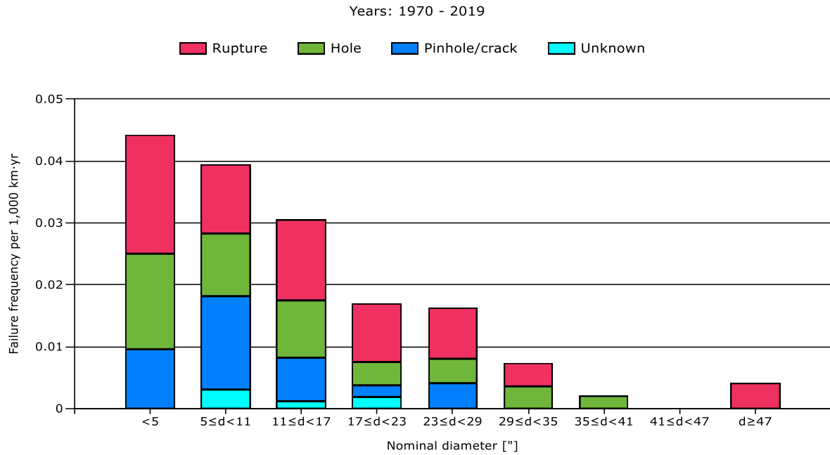
Figure 45: Relationship ground movement, size of leak and diameter (1970-2019)
