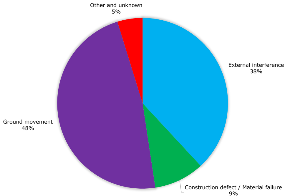
Figure 19: Distribution for incidents with leak size rupture (2010-2019)
