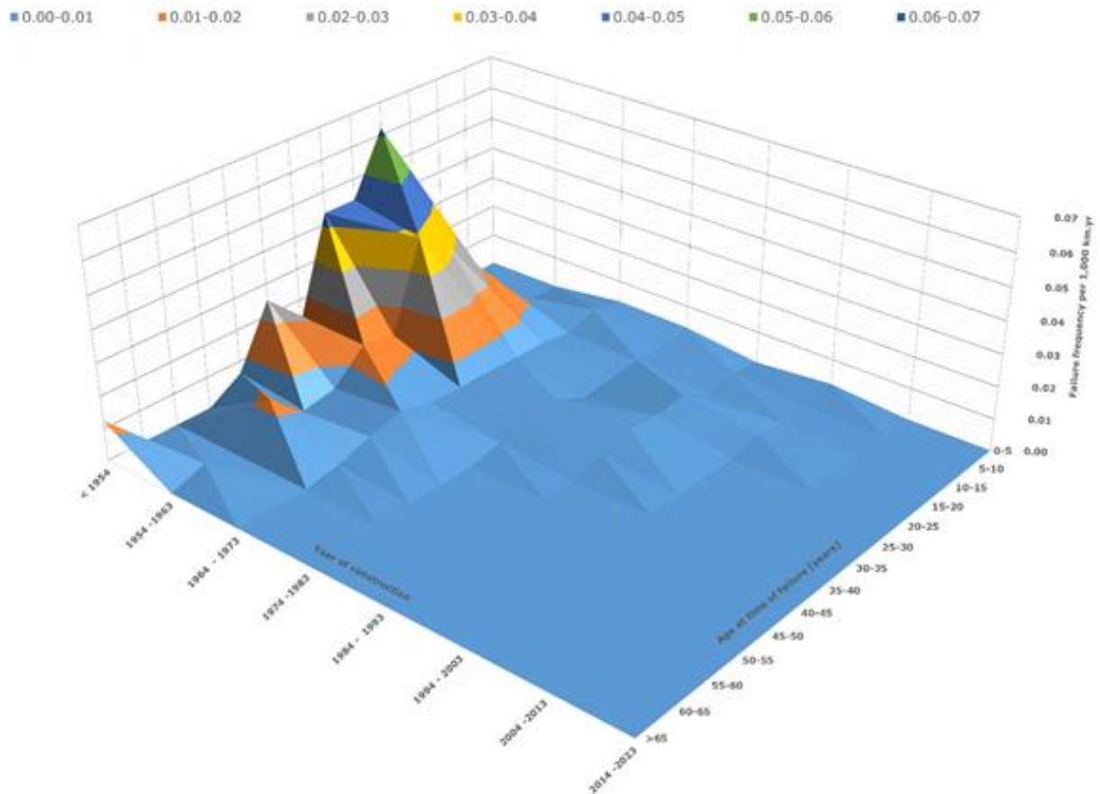
Figure 52: 3D plot of failure frequency of corrosion incidents and the age at the time of failure
