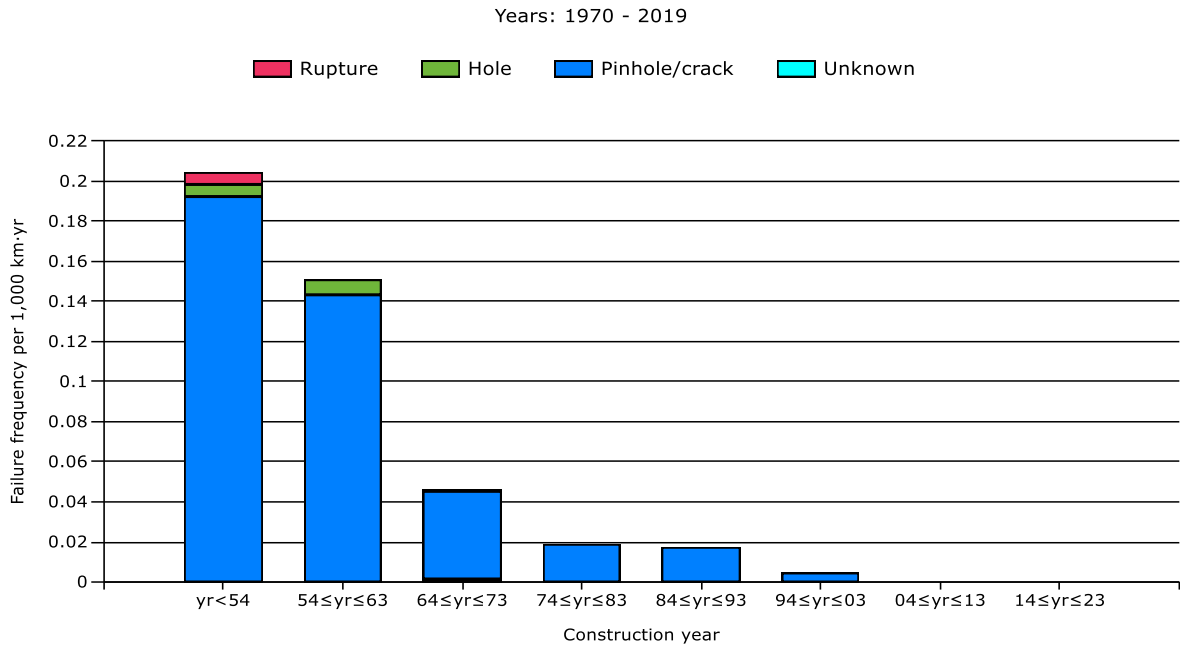
Figure 31: Relationship corrosion, size of leak and year of construction (1970-2019)
