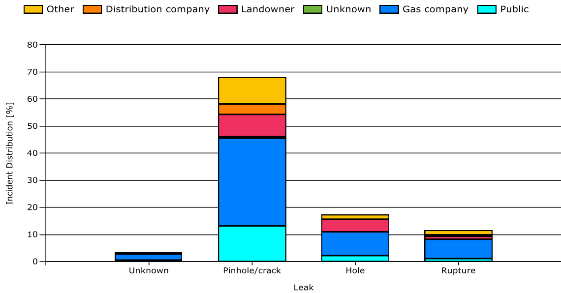
Figure 56: Detection of incidents per leak size (2010-2019)
