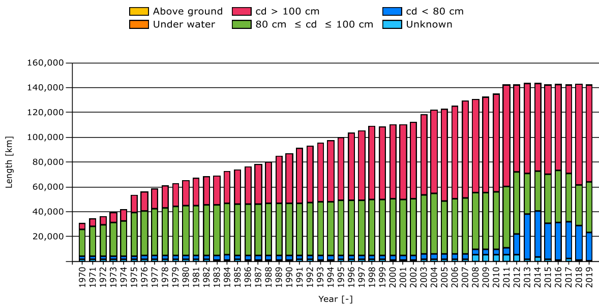
Figure 5: Total length per depth of cover (cd)
