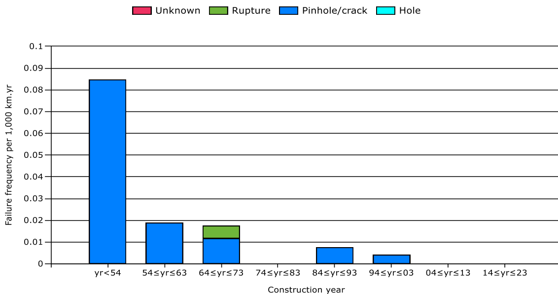
Figure 42: Relationship material failure, size of leak and year of construction (2010-2019)
