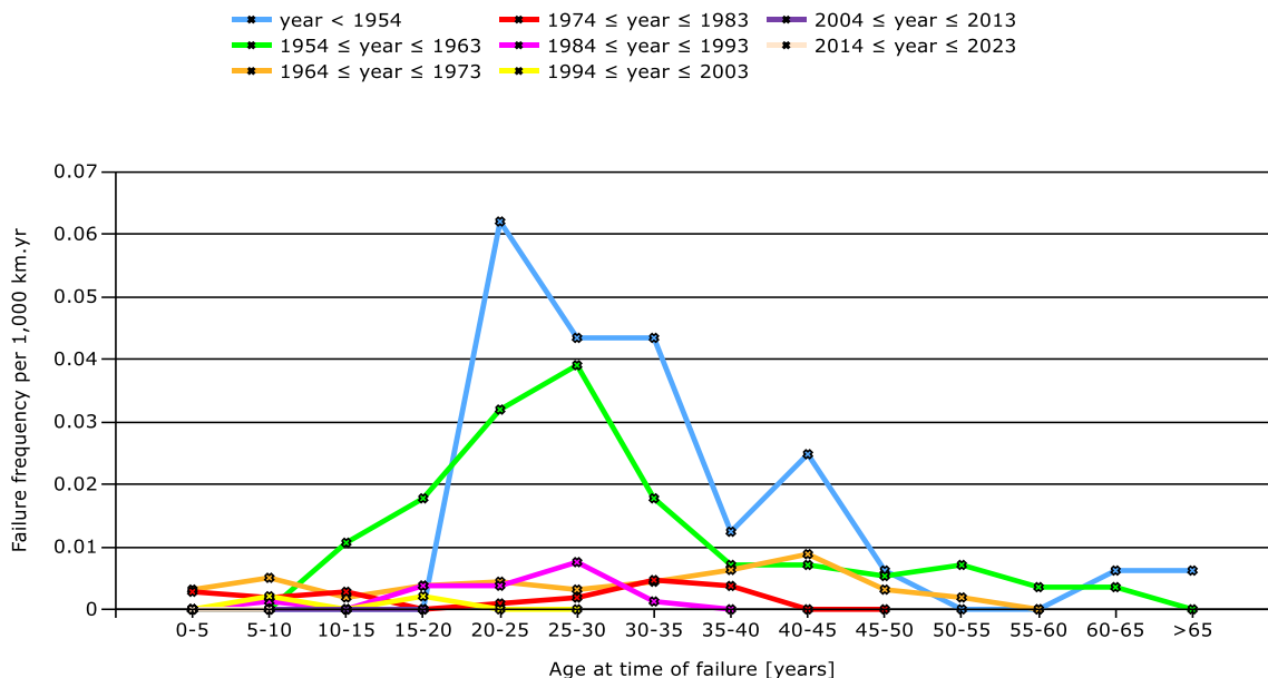
Figure 51: Relationship failure frequency of corrosion incidents and the age at the time of failure
