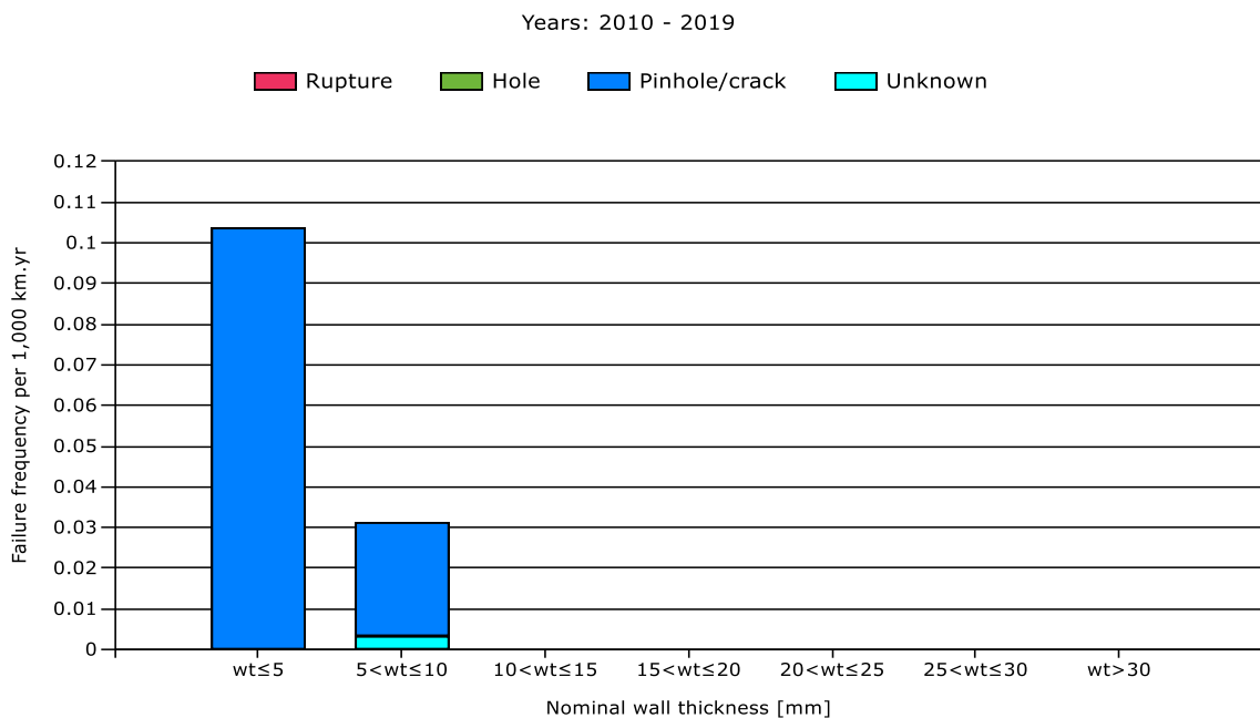
Figure 36: Relationship corrosion, size of leak and wall thickness (wt) (2010-2019)
