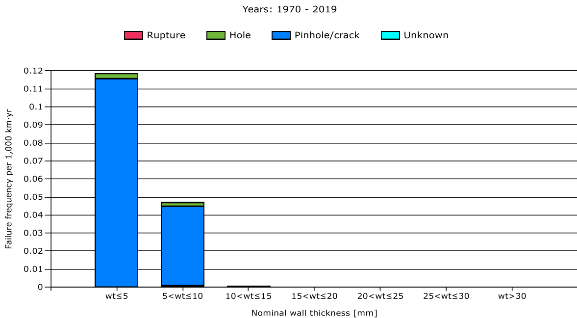
Figure 35: Relationship corrosion, size of leak and wall thickness (wt) (1970-2019)
