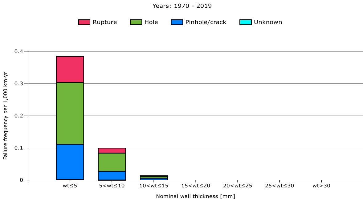
Figure 29: Relationship external interference, leak size and wall thickness (wt) (1970-2019)
