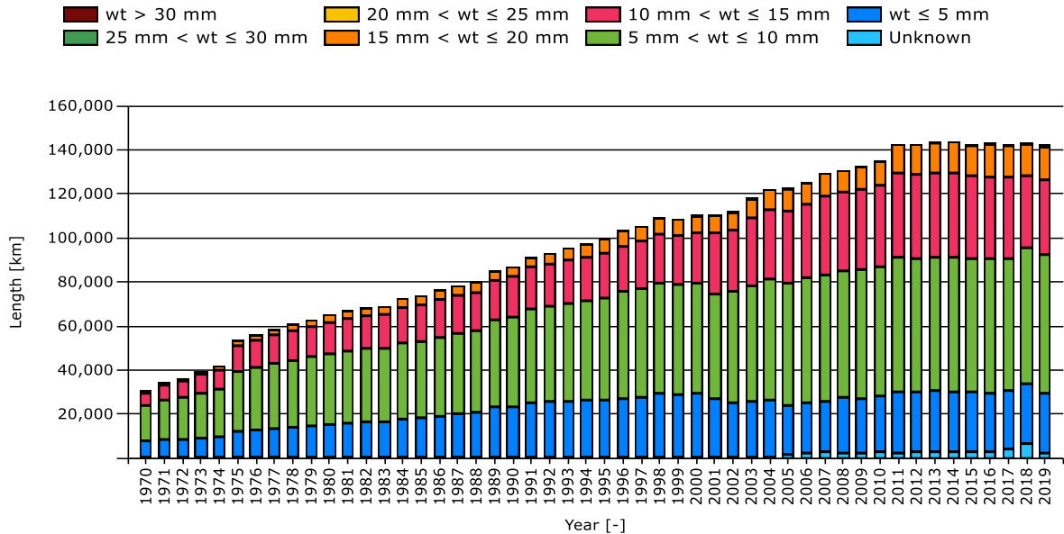
Figure 6: Total length per wall thickness (wt)
