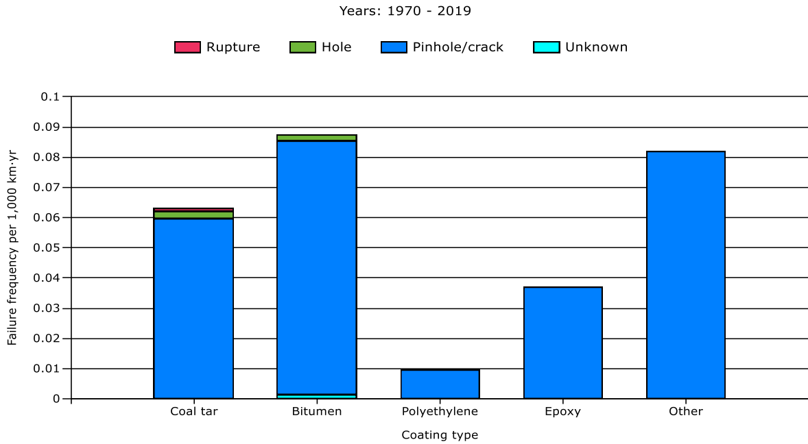
Figure 33: Relationship corrosion, size of leak and most common type of coating (1970-2019)
