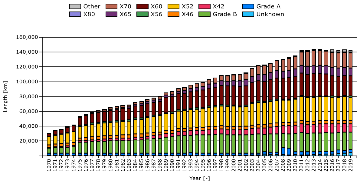
Figure 7: Total length per grade of material
