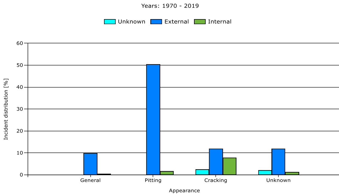
Figure 37: Breakdown of corrosion incidents on basis of location and appearance (1970-2019)
