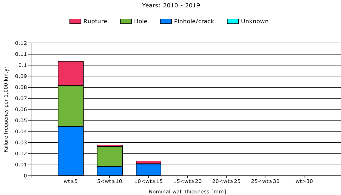
Figure 30 : Relationship external interference, size of leak and wall thickness (wt) (2010-2019)
