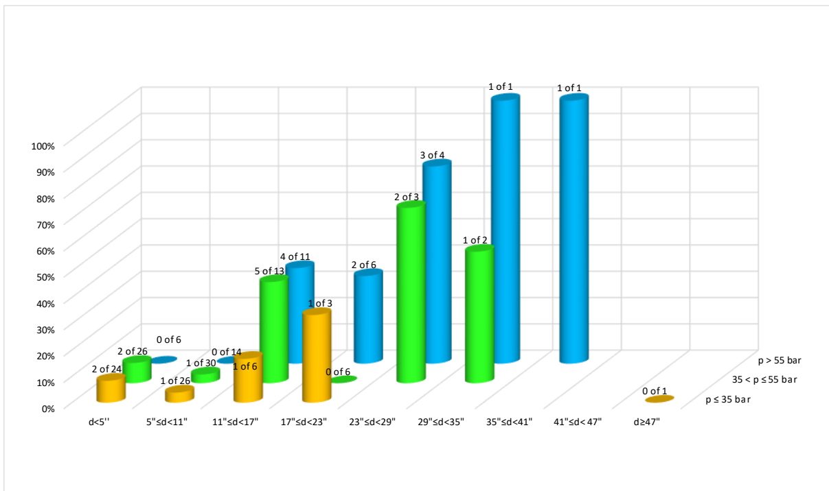
Figure 53: Percentages ruptures that ignited subdivided in diameter and pressure (1970-2019)
