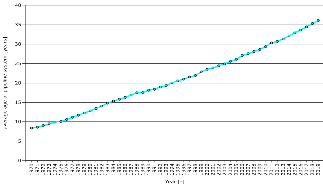
Figure 10: Average age of the pipeline system
