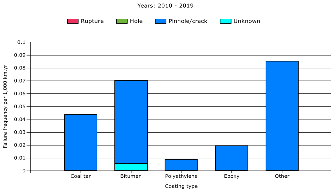
Figure 34: Relationship corrosion, size of leak and most common type of coating (2010-2019)
