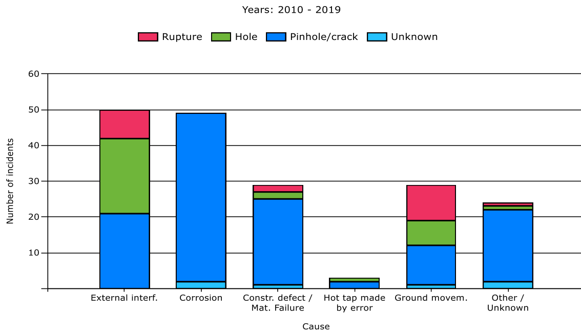
Figure 22: Number of incidents per cause in the period of 2010 to 2019
