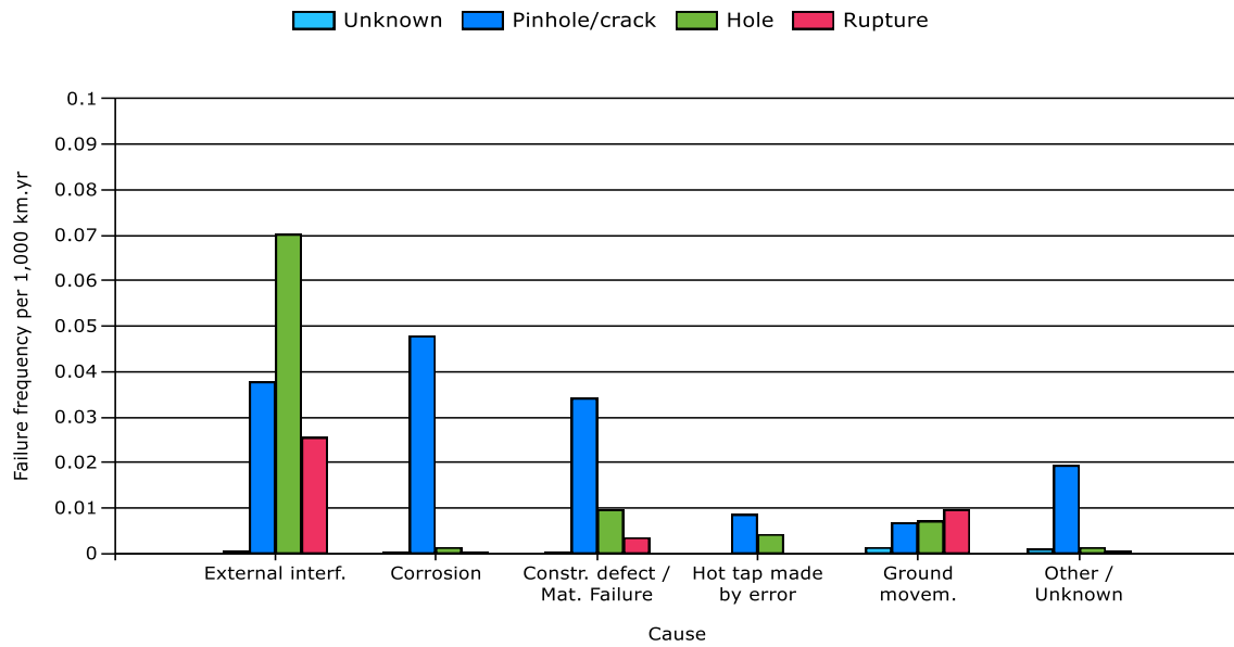
Figure 20: Relationship primary failure frequency, cause and size of leak (1970-2019)
