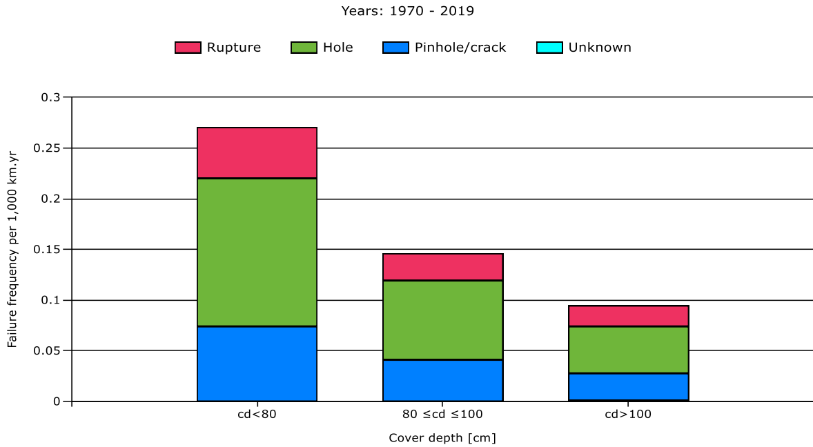
Figure 26: Relationship external interference, leak size and depth of cover (cd) (1970-2019)
