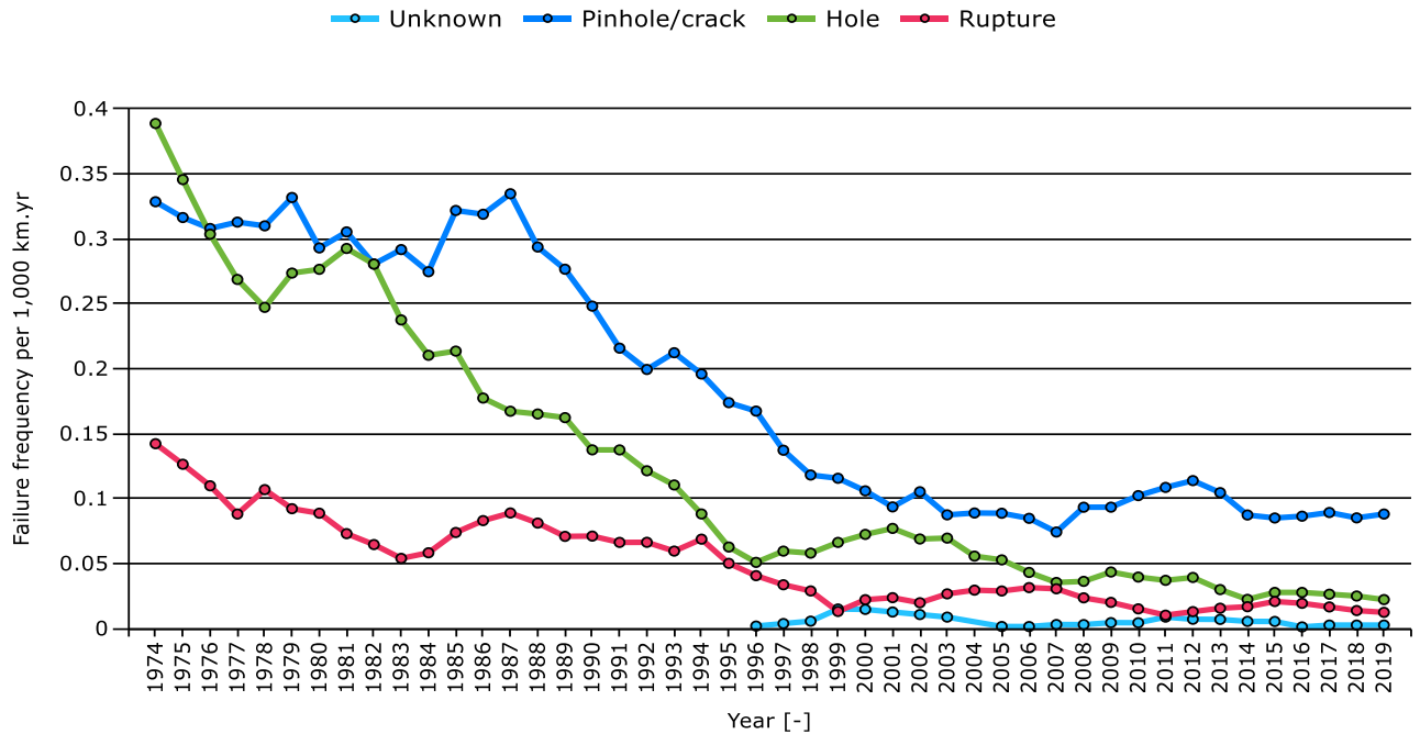
Figure 16: Primary failure frequency (five year moving average) per leak size
