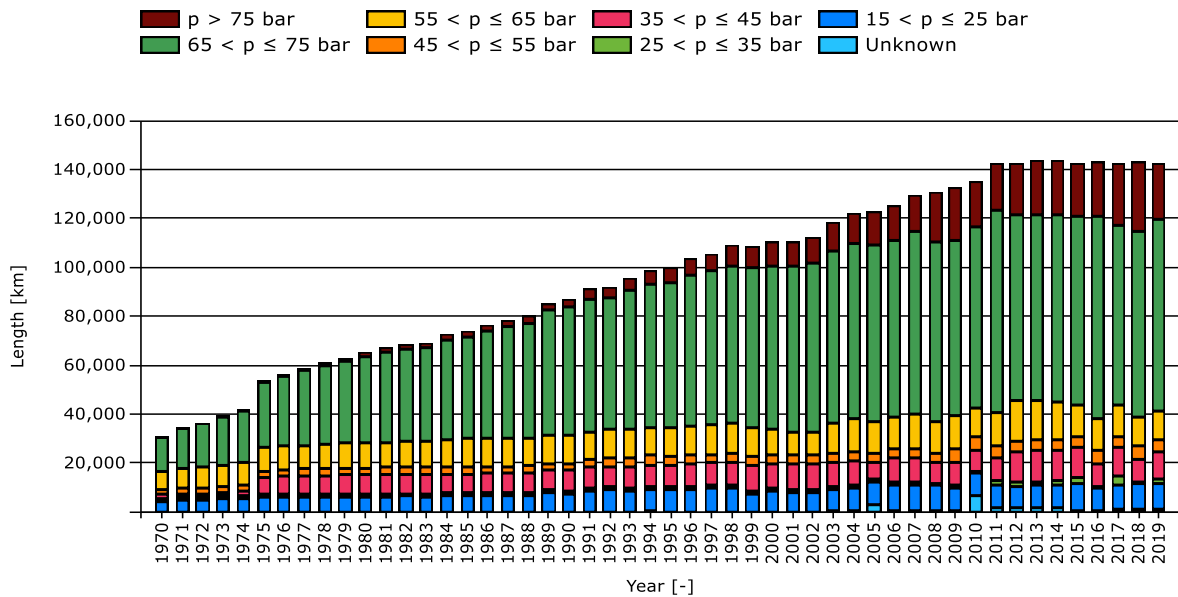
Figure 8: Total length per Maximum Operating Pressure (p)
