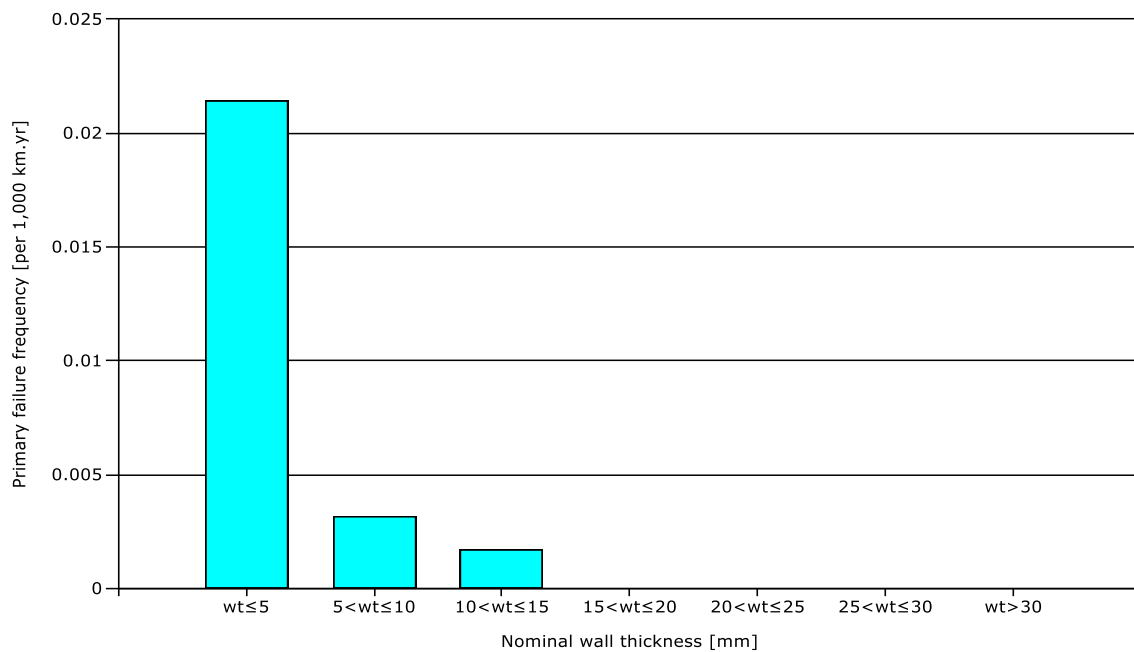
Figure 49: Relation wall thickness and failure frequency of incidents caused by lightning
