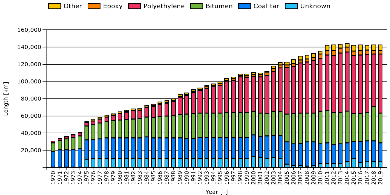
Figure 4: Total length per type of coating
