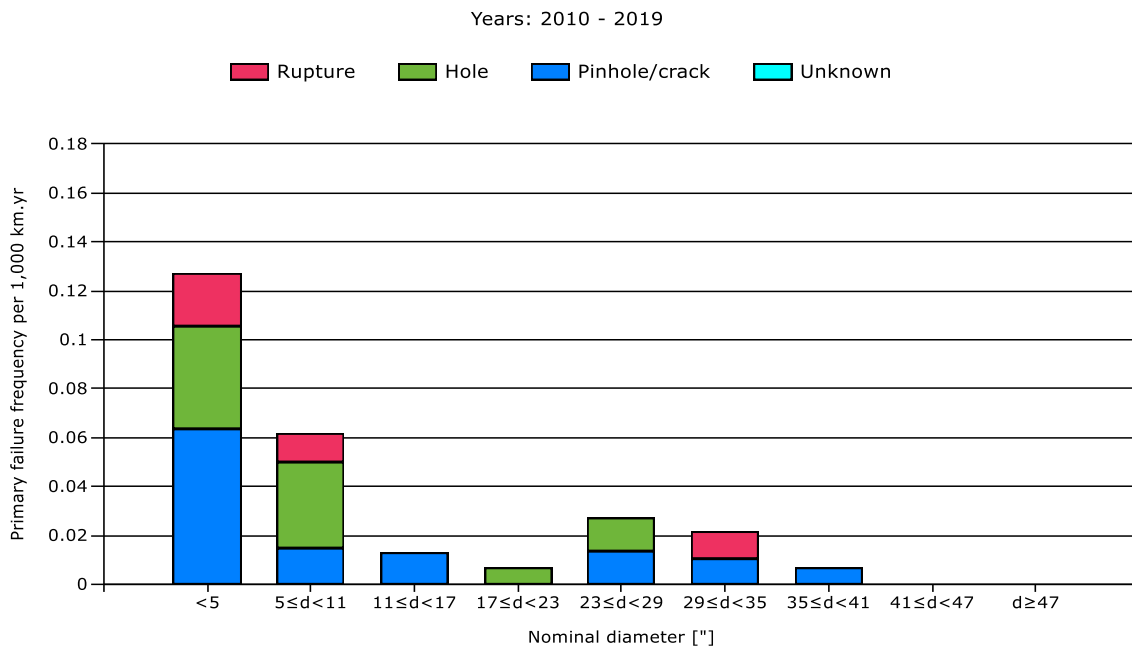
Figure 25: Relationship external interference, leak size and diameter (d) (2010-2019)
