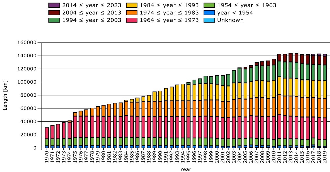
Figure 3: Total length per year of construction
