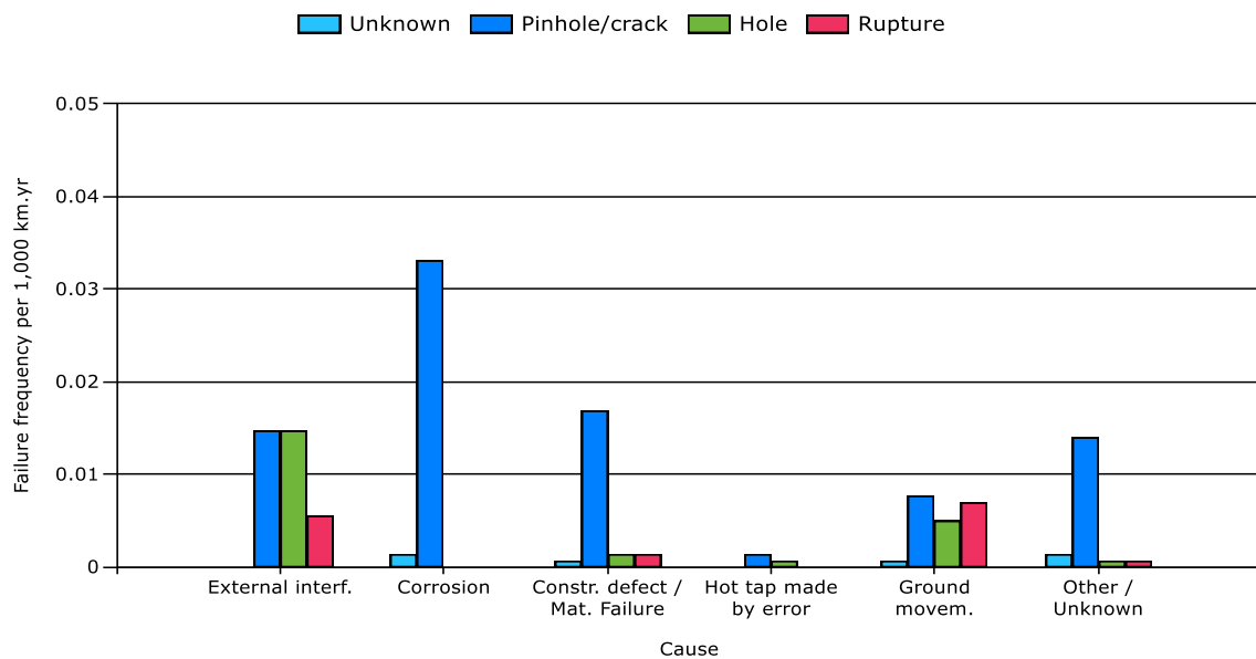
Figure 21: Relationship primary failure frequency, cause and size of leak (2010-2019)
