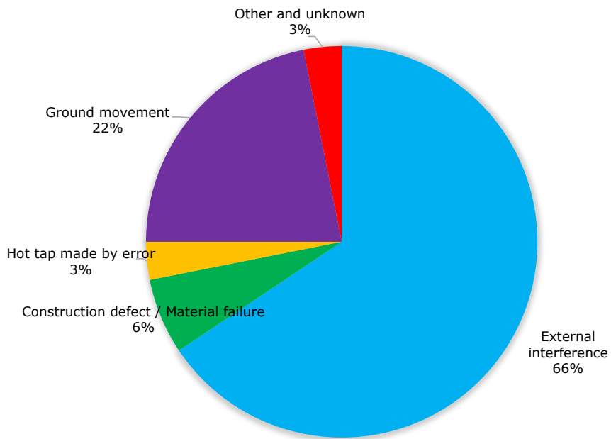
Figure 17: Distribution for incidents with leak size pinhole/crack (2010-2019)
