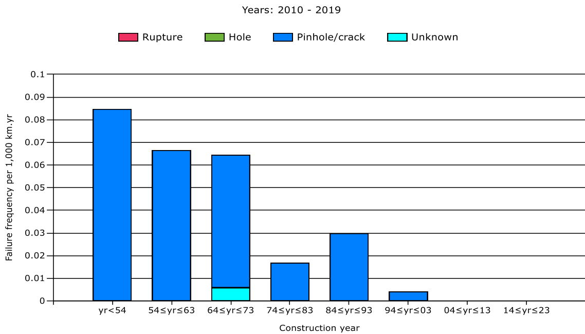
Figure 32: Relationship corrosion, size of leak and year of construction (2010-2019)
