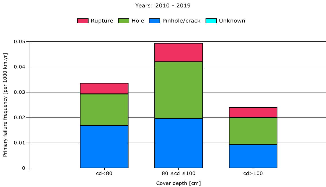
Figure 27: Relationship external interference, leak size and depth of cover (cd) (2010-2019)
