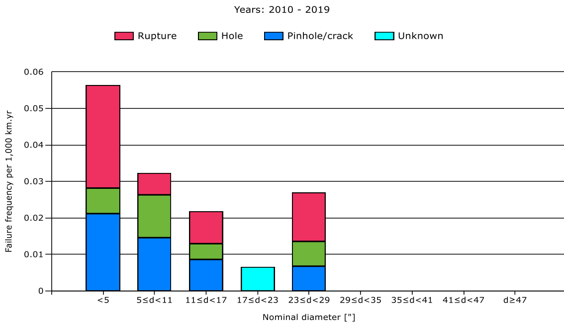
Figure 46: Relationship ground movement, size of leak and diameter (2010-2019)
