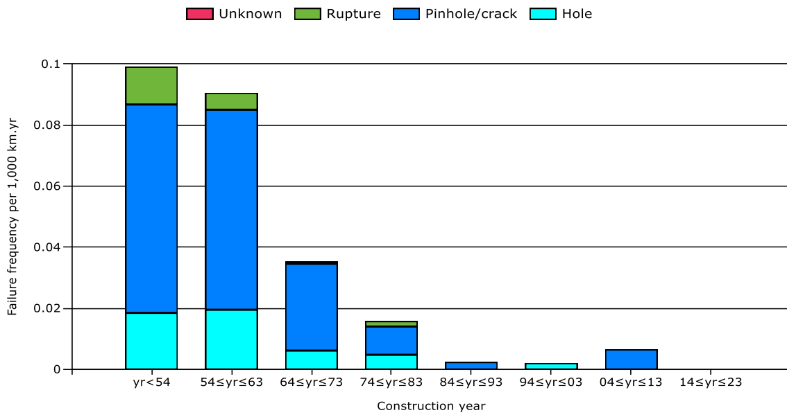
Figure 39: Relationship construction defect, size of leak and year of construction (1970-2019)
