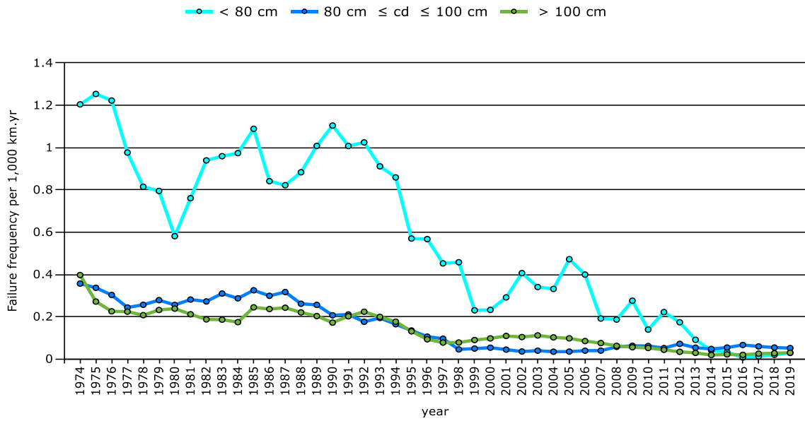
Figure 28: Failure frequency of external interference (five year moving average) and depth of cover
