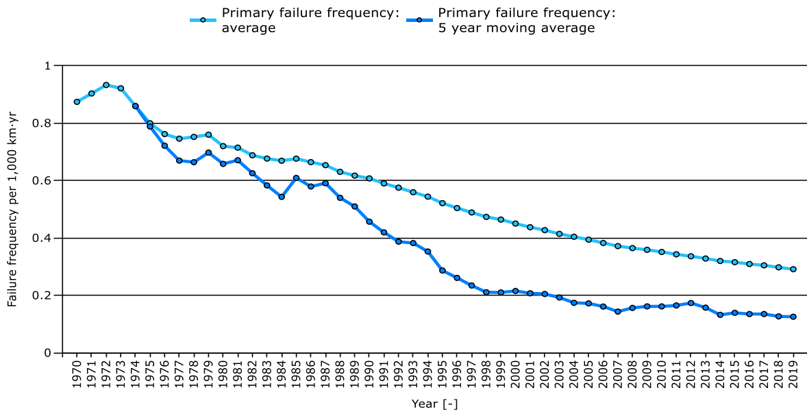
Figure 13: Primary failure frequencies
