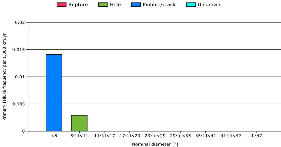
Figure 44: Relationship hot tap made by error, leak size and diameter (2010-2019)
