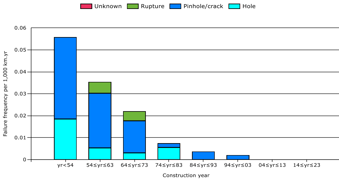
Figure 41: Relationship material failure, size of leak and year of construction (1970-2019)
