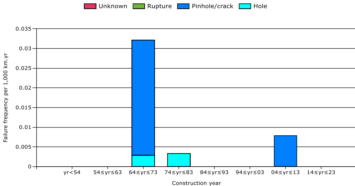
Figure 40: Relationship construction defect, size of leak and year of construction (2010-2019)
