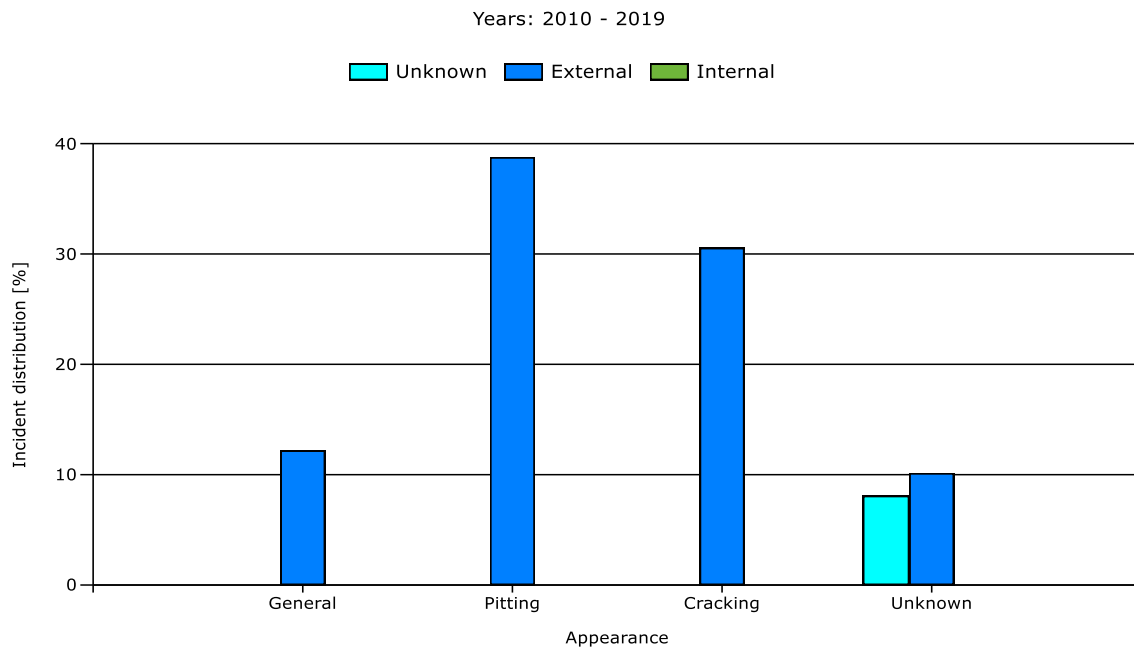
Figure 38: Breakdown of corrosion incidents on basis of location and appearance (2010-2019)
