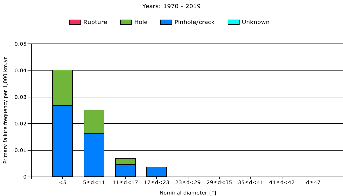
Figure 43: Relationship hot tap made by error, leak size and diameter (1970-2019)
